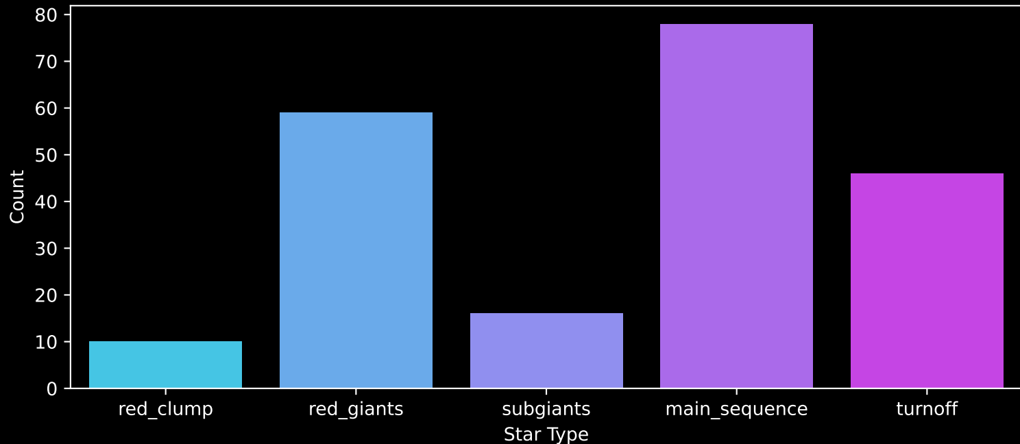
APOGEE DR17 Field: [176+29_MGA] Count plot of Star Type
