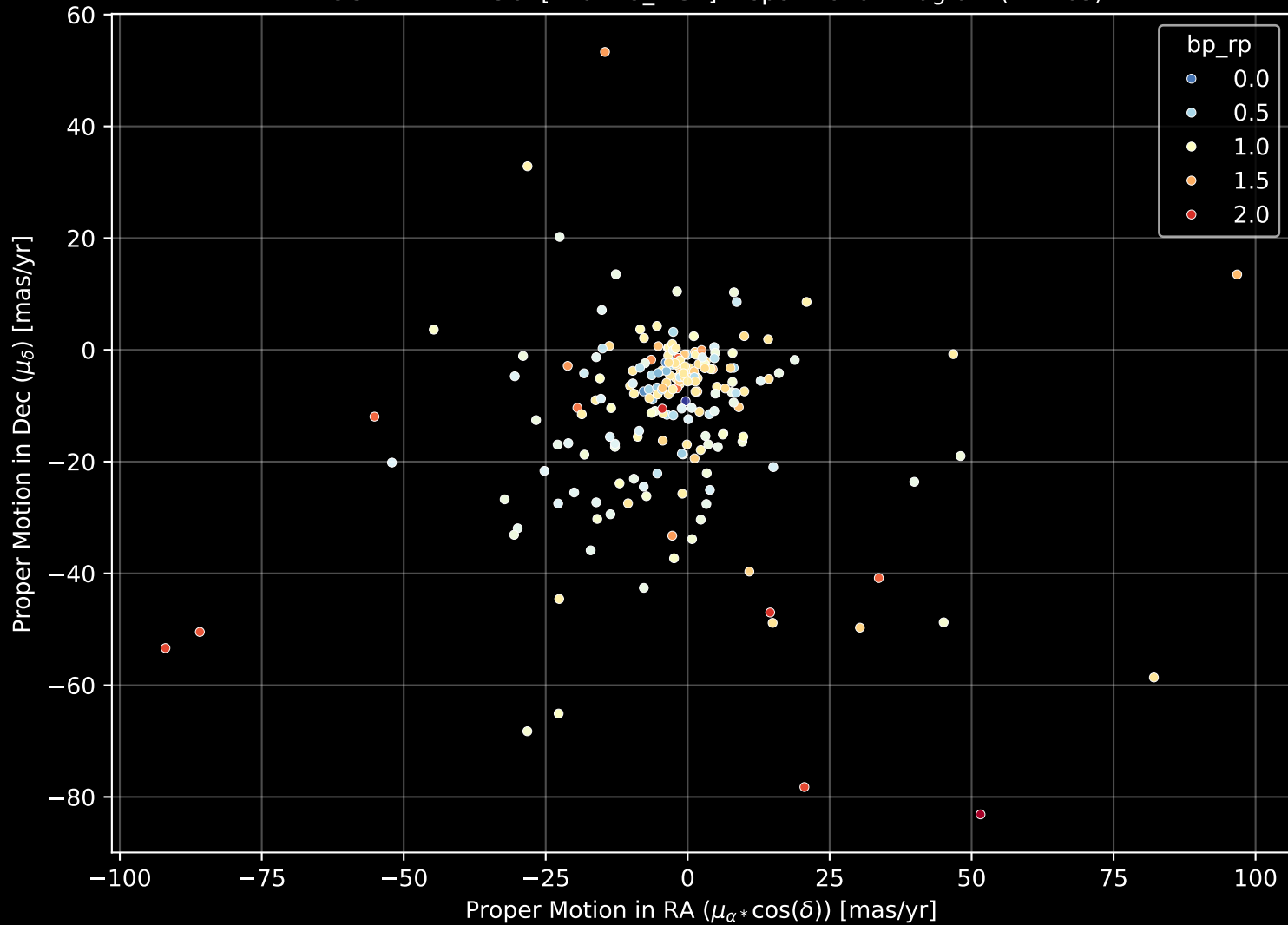
APOGEE DR17 Field: [176+29_MGA] Proper Motion Diagram (n= 209)
