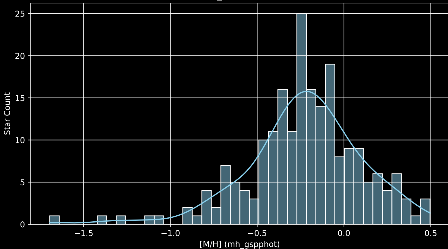
APOGEE DR17 Field: [176+29_MGA [M/H] (mh_gspphot) (n= 209)
