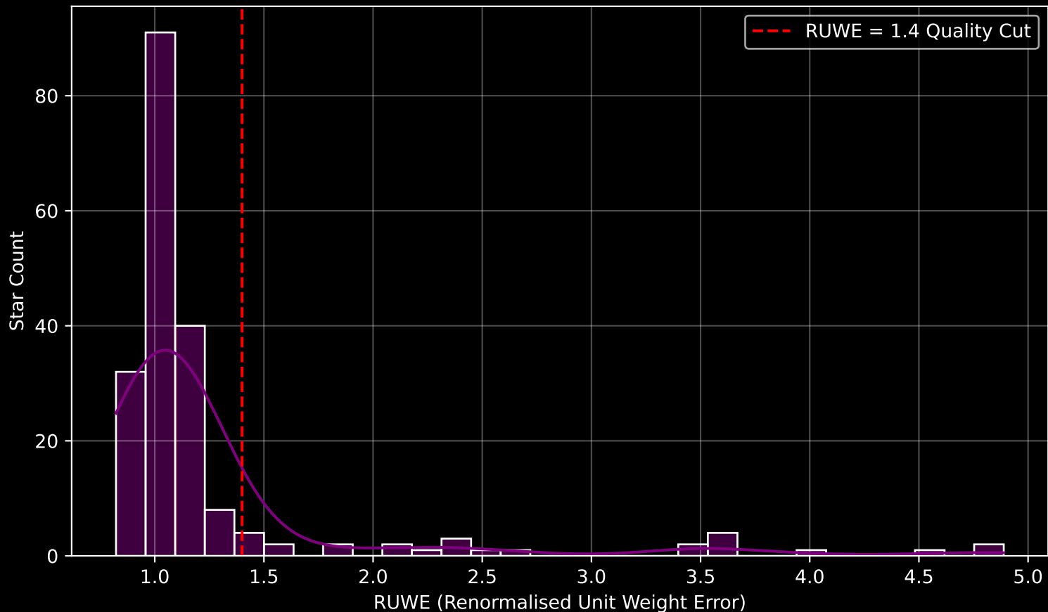
GAPOGEE DR17 Field [176+29_MGA] RUWE Distribution (n= 197)
