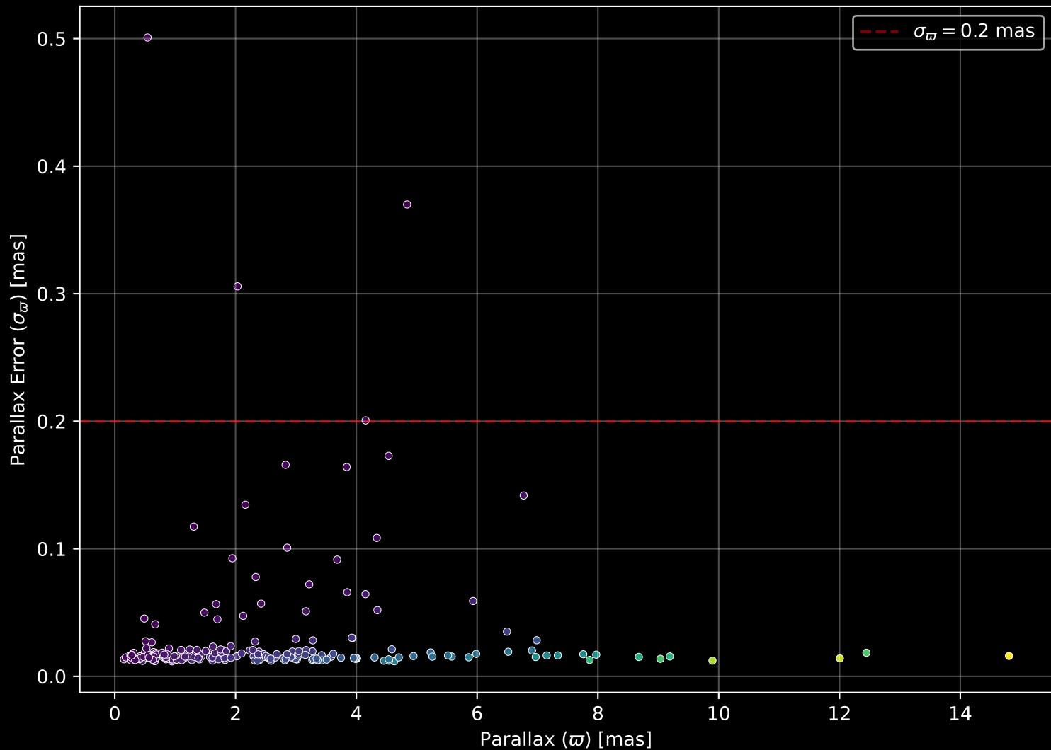
APOGEE DR17 Field: [176+29_MGA] Parallax Quality (n= 209)
