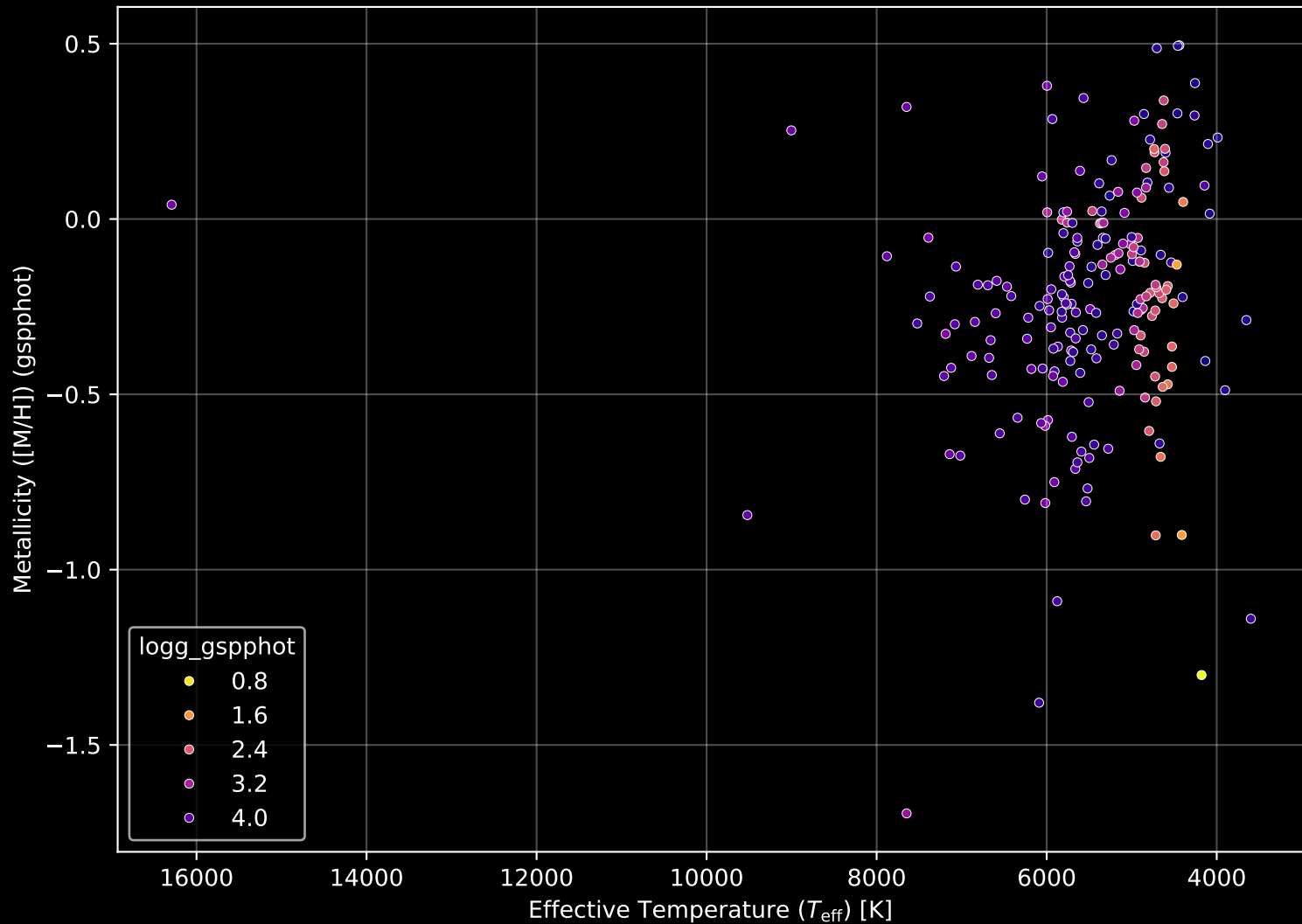
APOGEE DR17 Field: [176+29_MGA] Stellar Population Parameters (n= 209)
